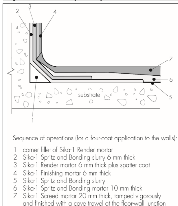
Figure 2 Formation of corner joint
