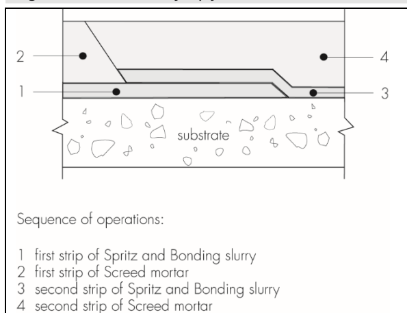
Figure 1 Formation of lap joint
