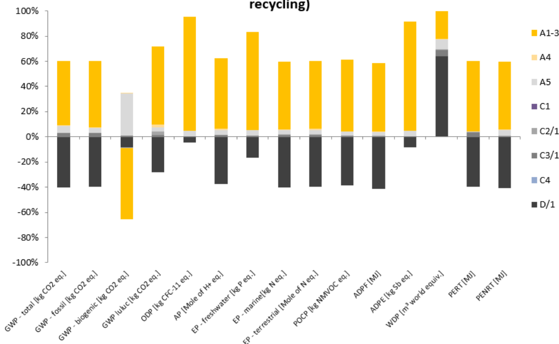
Relative contributions of the modules to the LCA categories and to primary energy use for 1 m 2 Sikaplan® SGmA-15 (100% material recycling)
